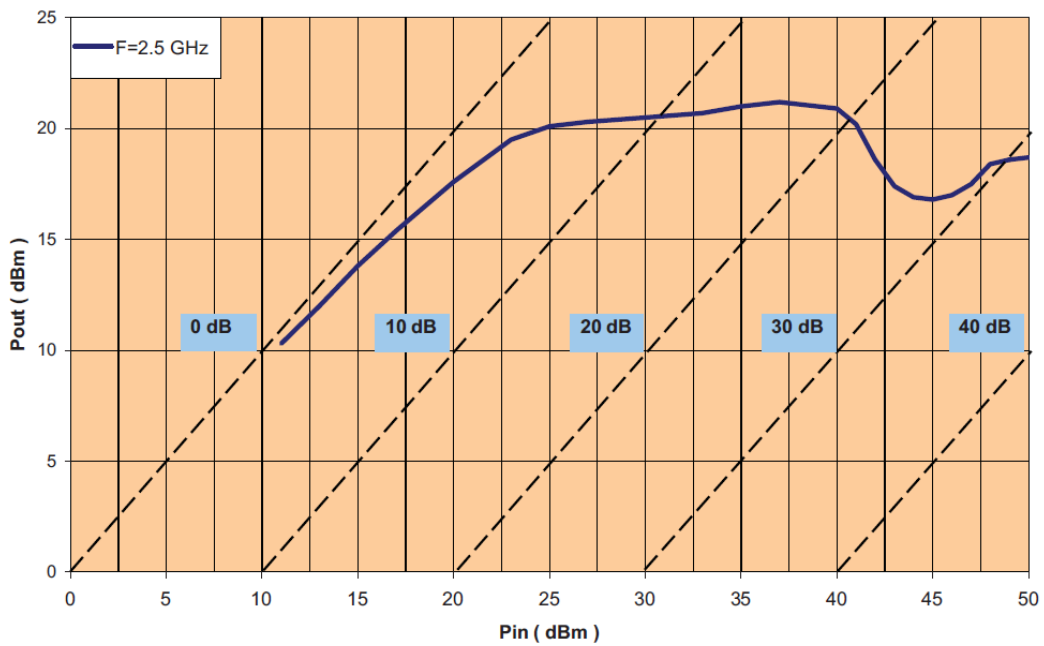
RFLM-202802QC-290 Flat Leakage CW Power Output vs CW Input Output
