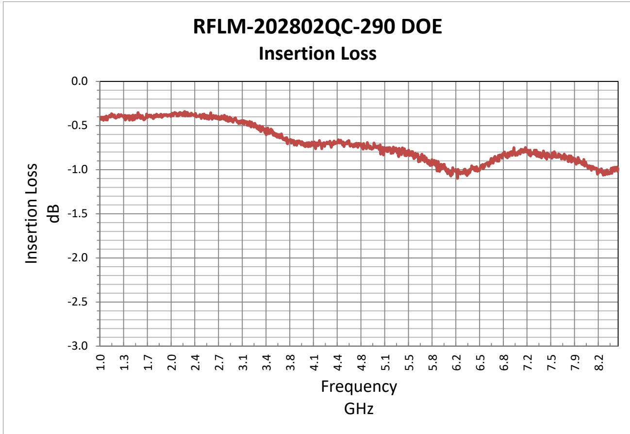
RFLM-202802QC-290 Insertion Loss vs Frequency
